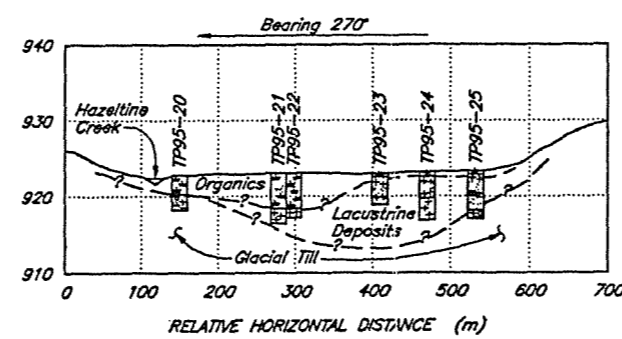
SECTION 1 1623.100 POLLEY LAKE DAM SITE
