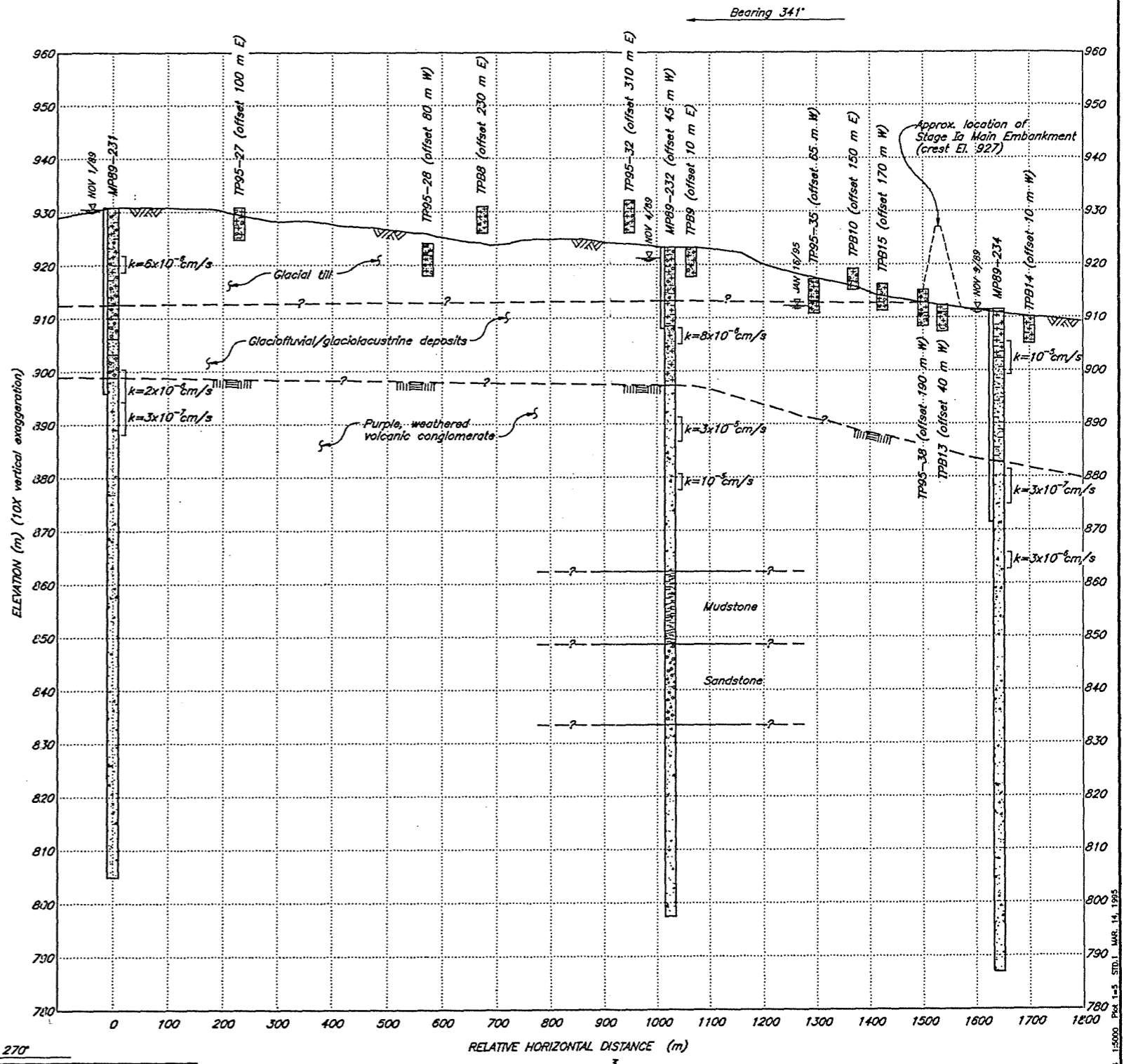
SECTION 3 1623.102 TAILINGS BASIN
