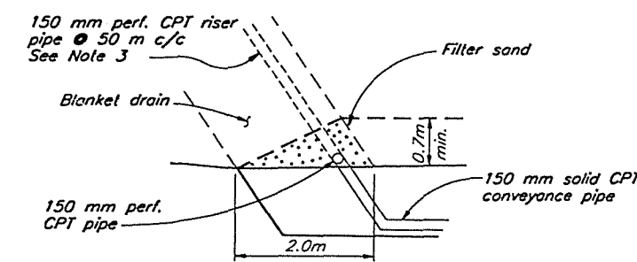
DETAIL C PERIMETER EMBANKMENT TOE DRAIN
