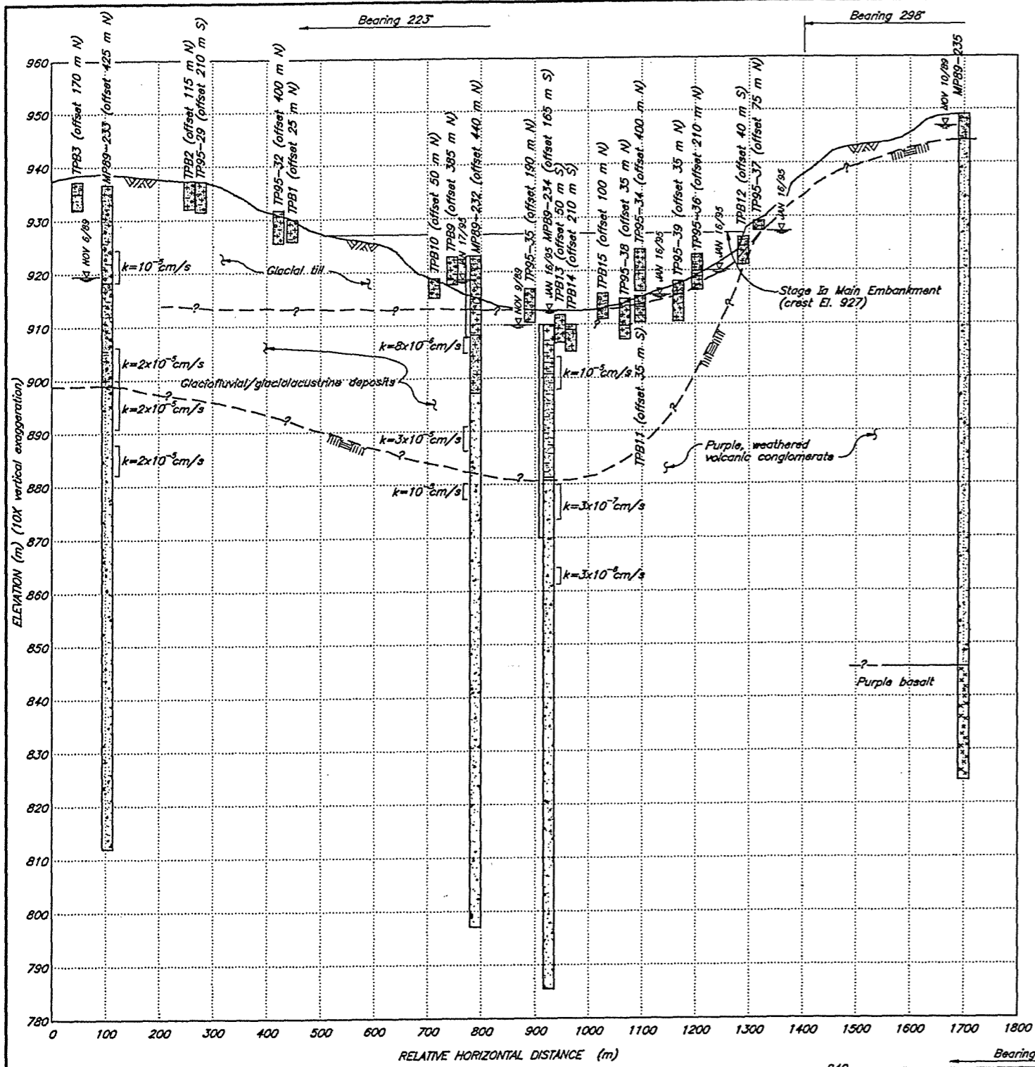
SECTION 2 1623.102 MAIN EMBANKMENT
